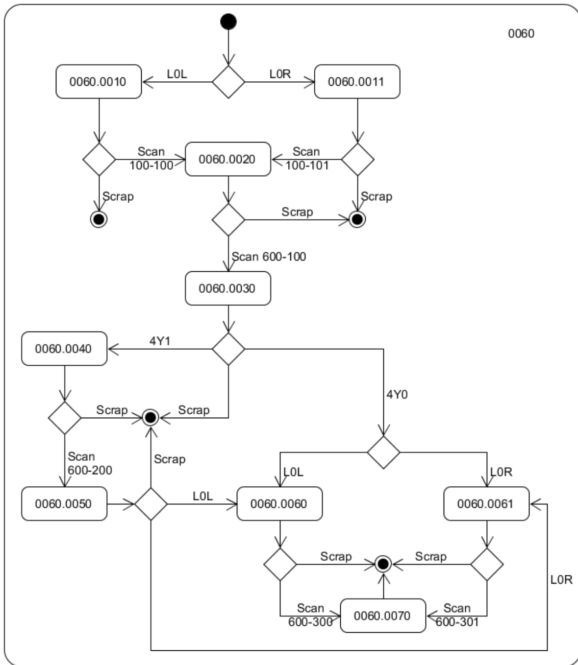
Figure 5 Process step 0060
