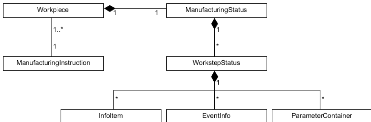
Figure 11 Workpiece
